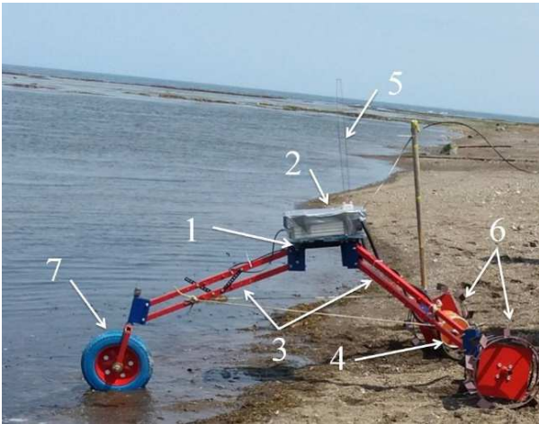
Fig. 2 Creeping Wave Platform (1) main structure, (2) watertight container, (3) arms to arms to adjust the posture of CWP, (4) stepping motor, (5) wire sensor, (6) driving wheels, (7) supporting wheel.
