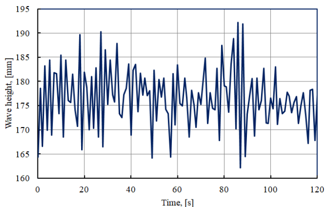
Fig. 5 An example of breaking waves recorded by the wire sensor
