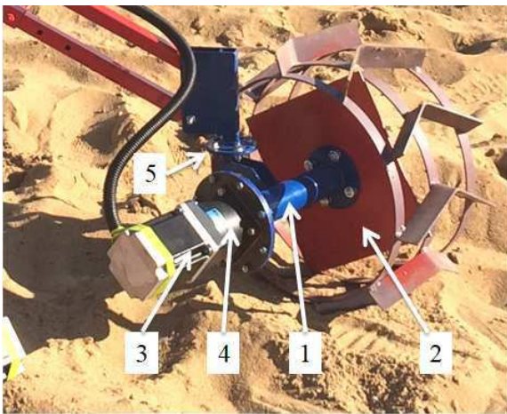
Fig. 3 Chassis of CWP (1) hub assembly, (2) wheel, (3) stepping motors, (4) bare gear box, (5) pivoting assembly
